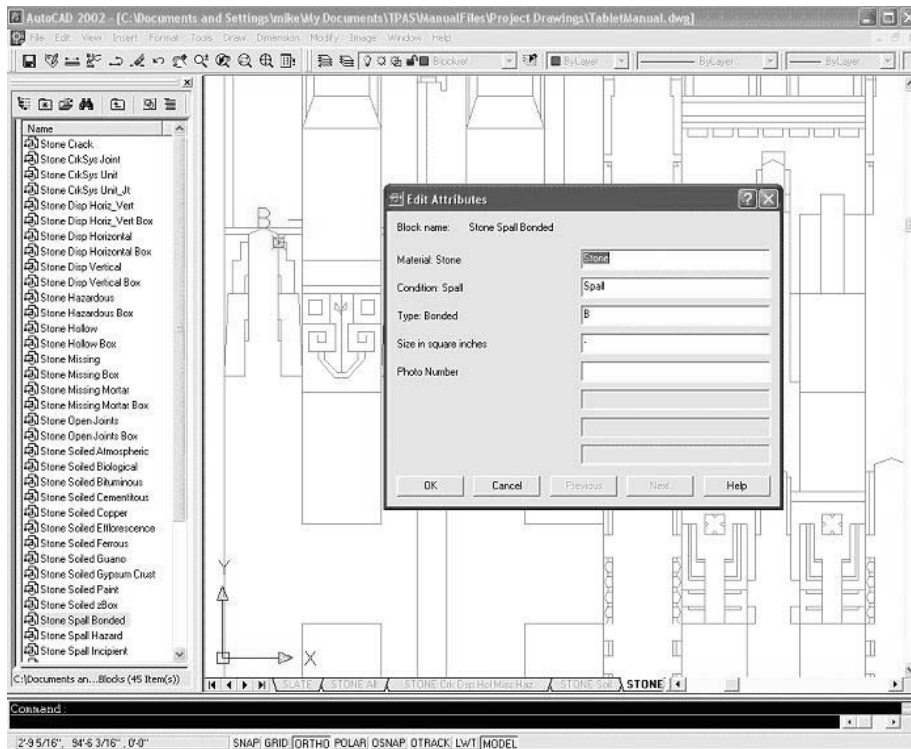
Fig. 3. When inserting a block attribute tag from the design center, the user drags the icon from the list at the left into the drawing, upon which the Edit Attributes dialog box prompts the user for information on the size of the condition in question (in square inches in this case).
